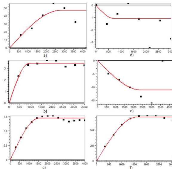
Figure 5: Variograms of the primary and two secondary variables, where a) shows the variogram of the well, b) shows the variogram of the angle stack amplitude, c) shows the variogram of the V_p/V_s ratio, d) shows the variogram of well and angle stack amplitude, e) shows the variogram of well and V_p/V_s ratio, and f) shows the variogram of angle stack amplitude and V_p/V_s ratio.
