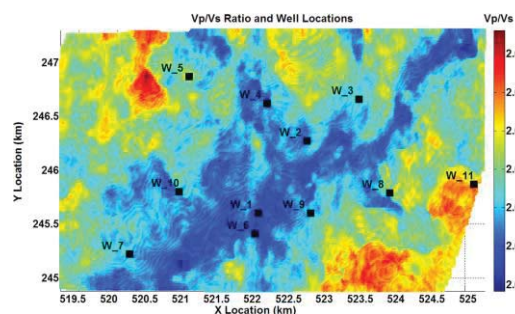
Figure 3: V_p/V_s ratio extracted from an inverted seismic volume using a window from 10ms above the top reservoir to 10ms below the base clastic formation.
