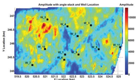
Figure 2: Seismic raw amplitude from an angle stack between 8^{\circ} and 29^{\circ} , using a window from 10ms above the reservoir to 10ms below the base clastic formation.
