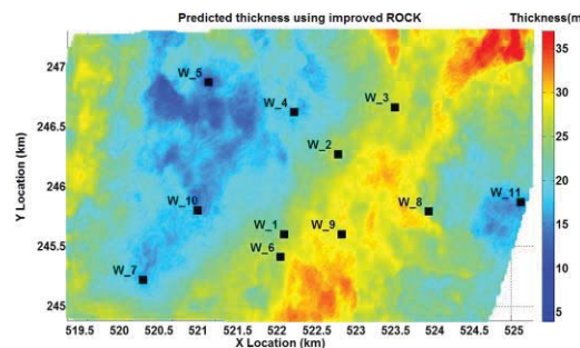
Figure 6: Predicted thickness and distribution of the reservoir formation using the improved ROCK method, obtained by considering thickness from the wells as the primary variable, and the angle stack amplitude and V_p/V_s ratio as two secondary variables.
