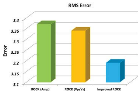
Figure 9: Root-mean-square errors using leave-one-out cross-validation for traditional ROCK with angle stack amplitude only, traditional ROCK with V_p/V_s ratio only, and the improved ROCK with these two attributes.
