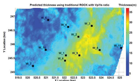
Figure 8: Predicted thickness and distribution of the reservoir formation using traditional ROCK with only one secondary variable: V_p/V_s ratio.
