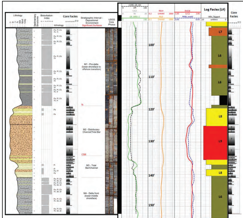
Figure 7: Detailed core description from one of the “Tier 1” HRA model wells (left), triple combo log suite from the same well with the synthetic core gamma ray shown as well as the core facies juxtaposed next to the log facies.
